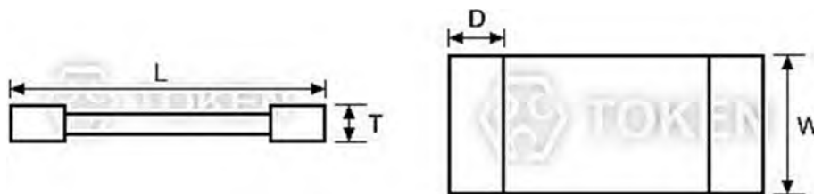
Chip 2512, 2010, 1206 Dimensions (LRC)
