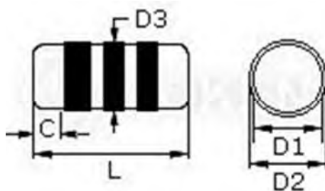
Carbon Film Low Noise MELF (RDM) Dimensions
