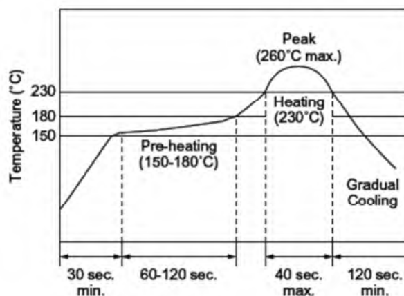
Reflow Solderings of Chip Type Ceramic Resonator
