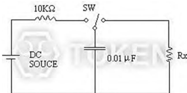
Test Circuit
