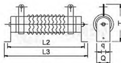
(DQ-B) G - Horizontal Mount
