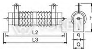
(DQBN) G - Horizontal Mount
