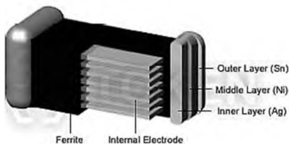
Surface Mount (TRMI) Material Construction
