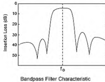
Figure-2 - Band pass Filter Characteristic
