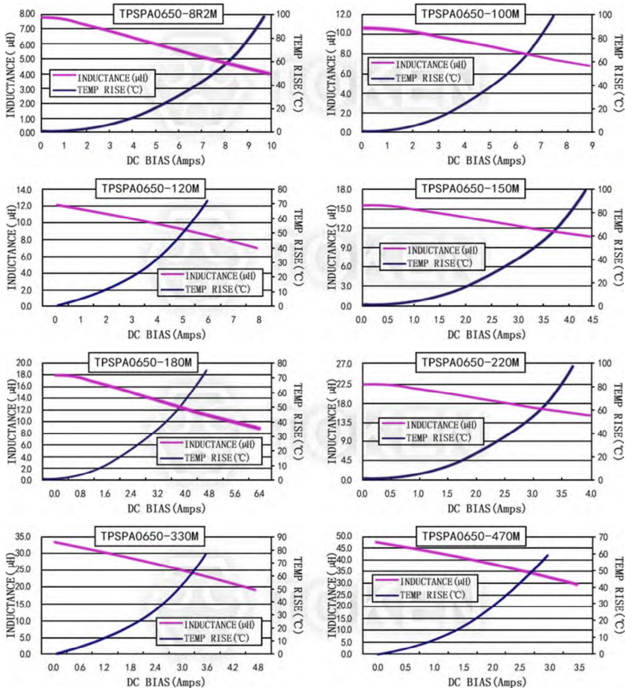
characteristics TPSPA0650-***M Series
