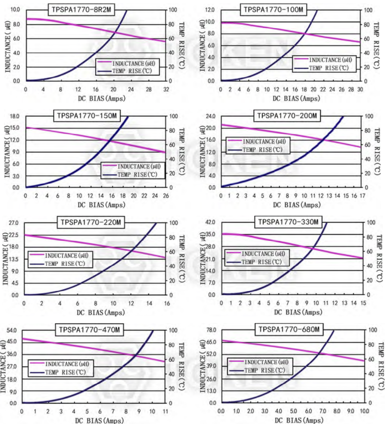
characteristics TPSPA1770-***M Series
