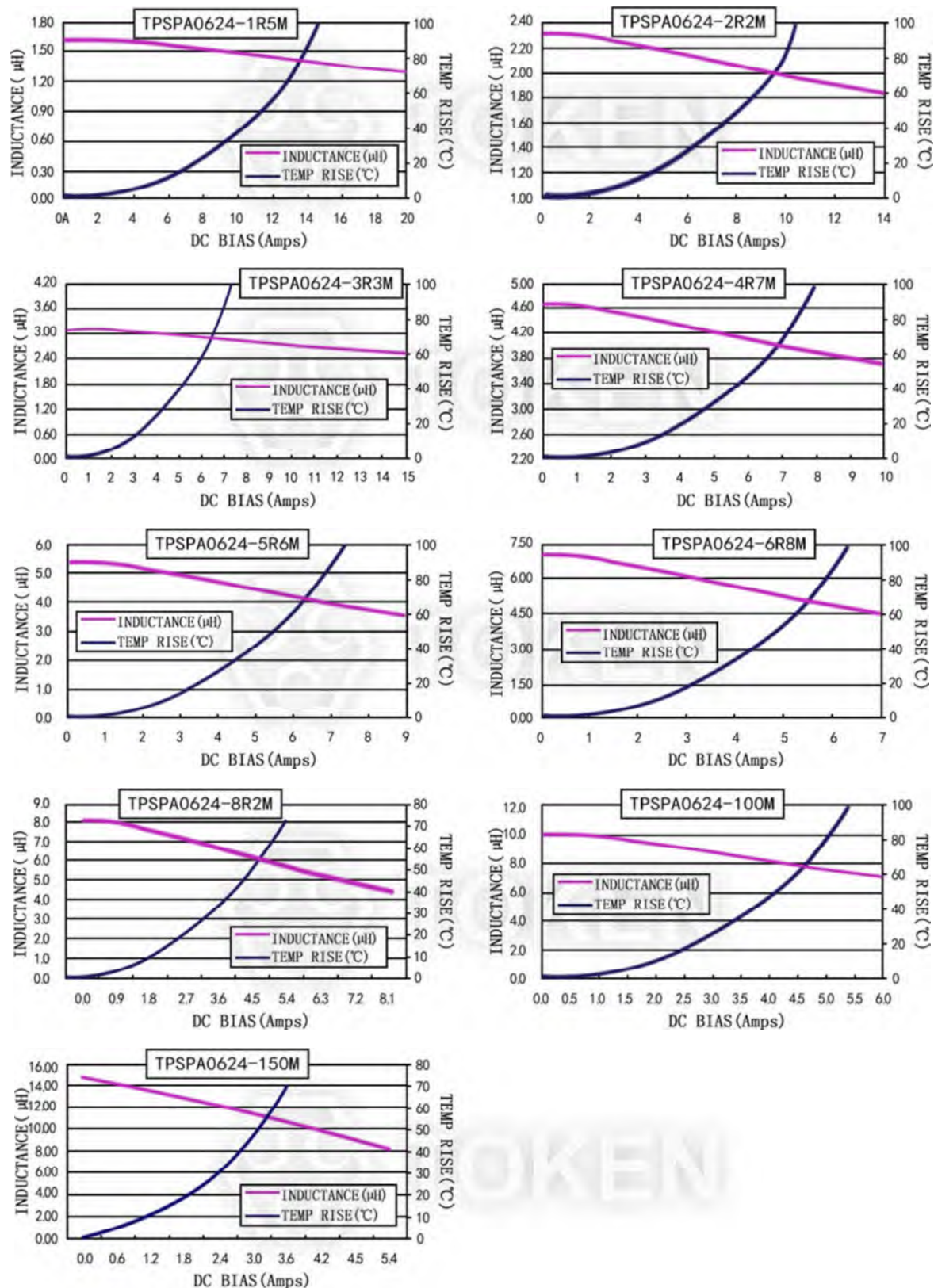
characteristics TPSPA0624-***M Series
