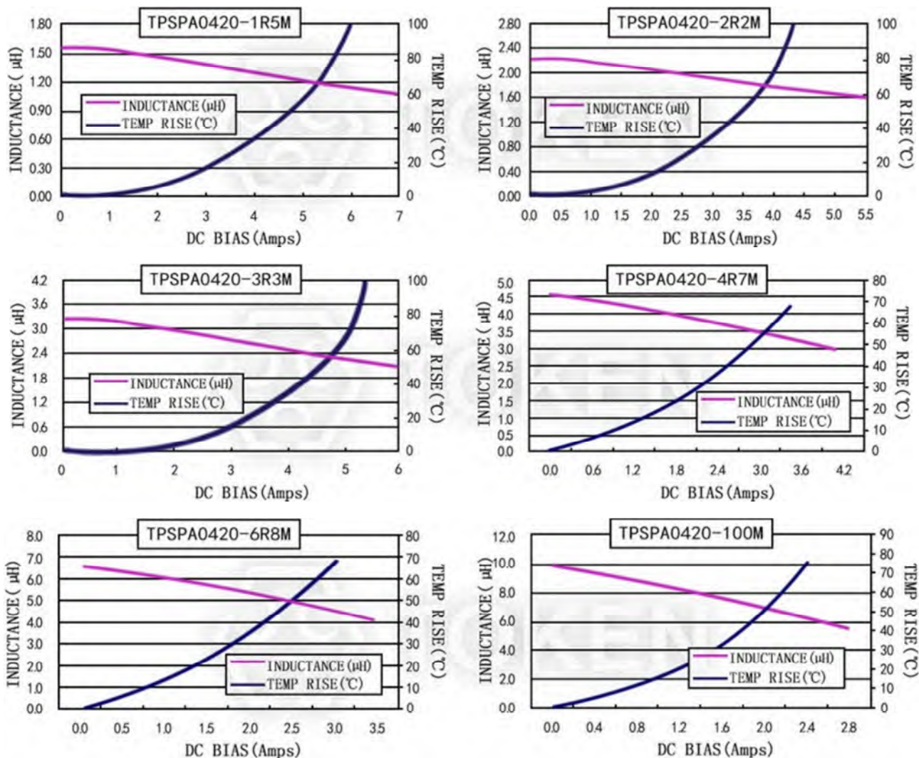
Current characteristics TPSPA0420-***M Series
