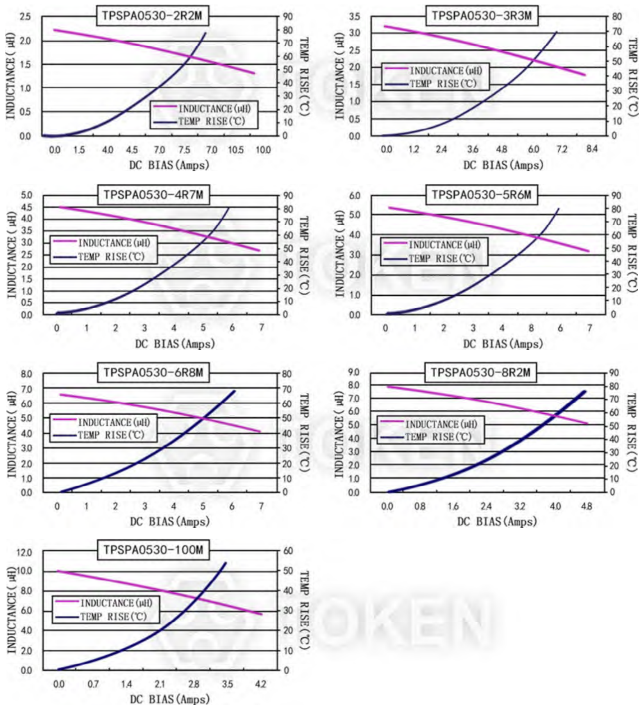
characteristics TPSPA0530-***M Series
