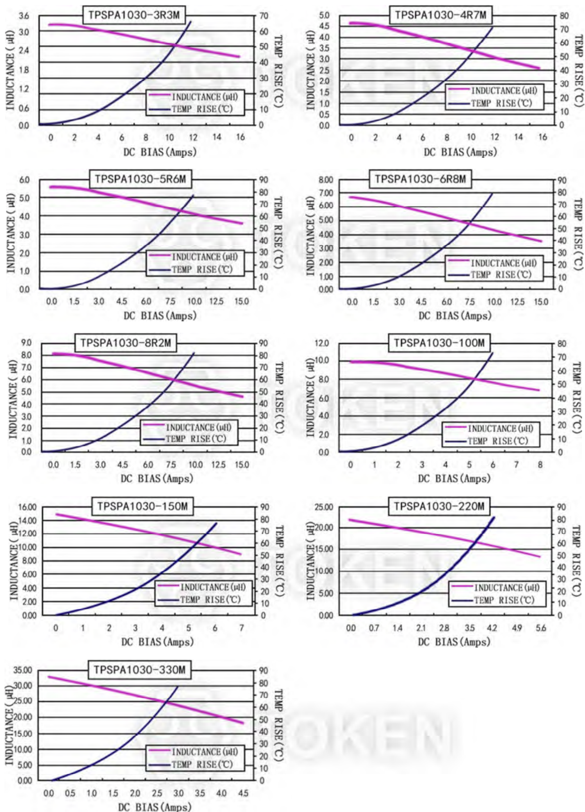
characteristics TPSPA1030-***M Series
