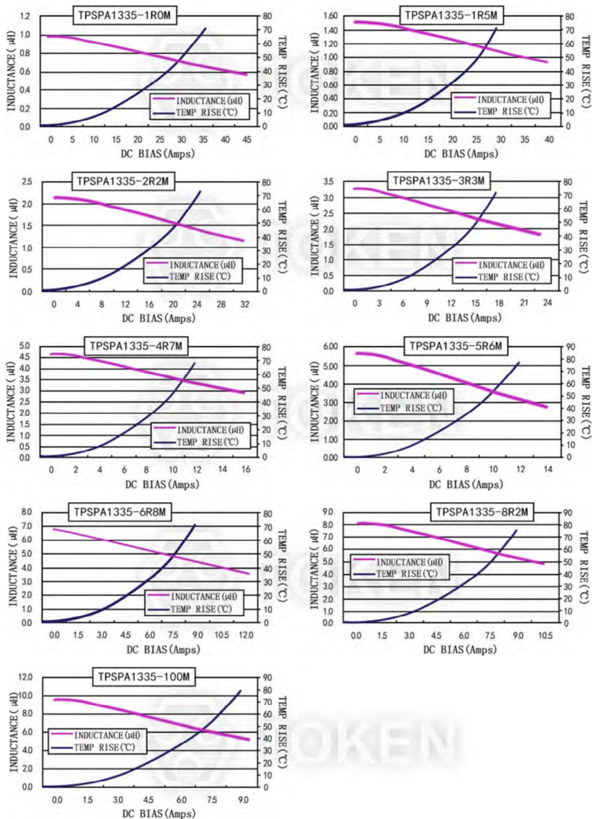
characteristics TPSPA1335-***M Series
