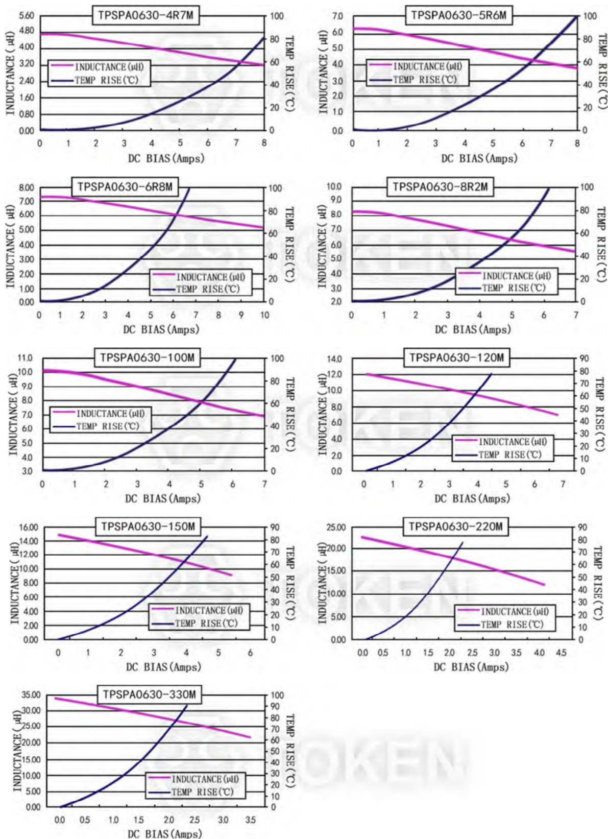
characteristics TPSPA0630-***M Series
