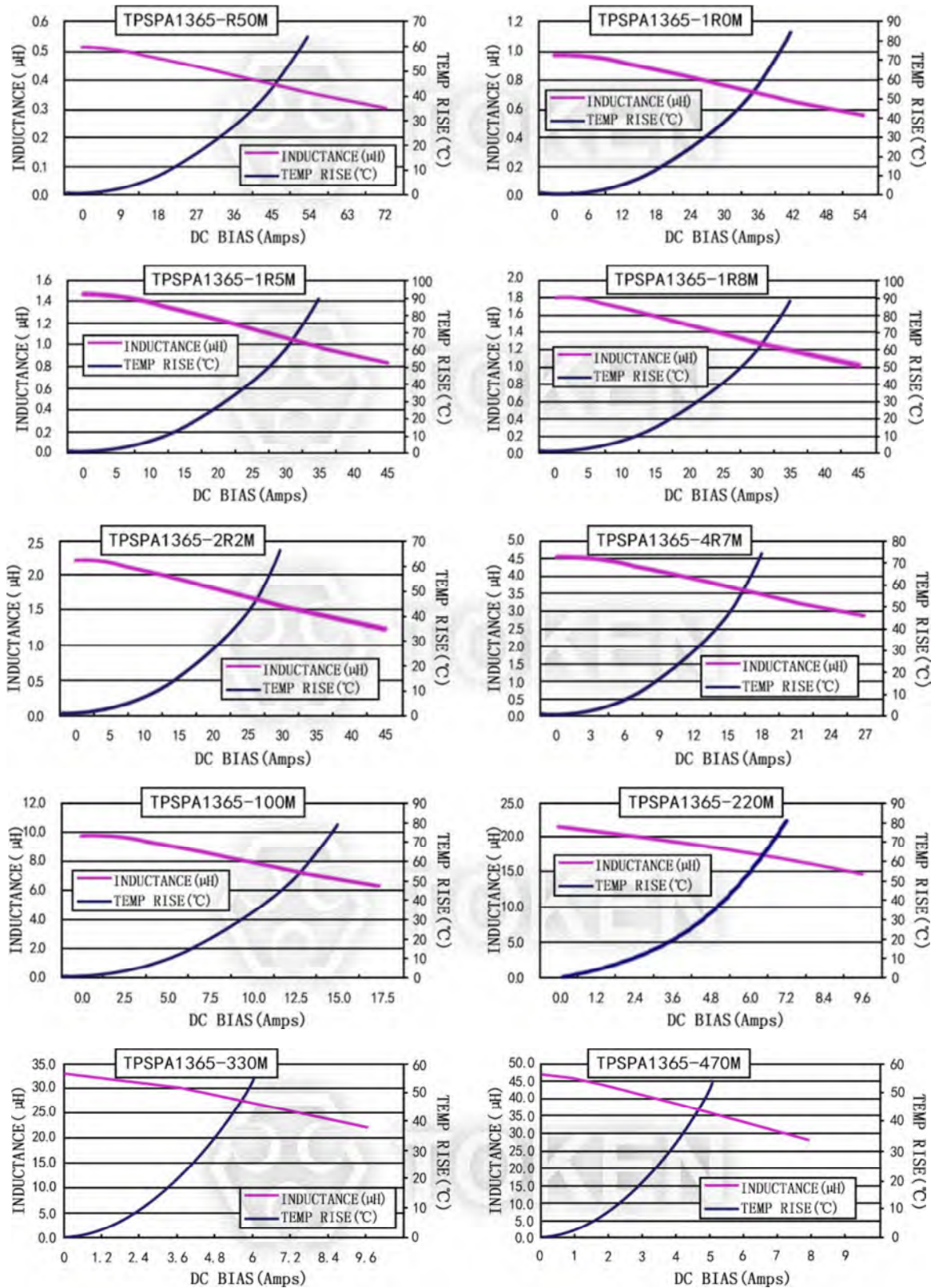
characteristics TPSPA1365-***M Series
