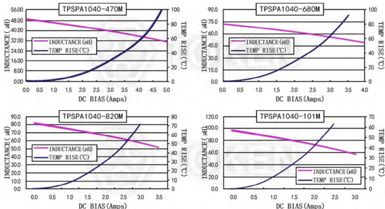
characteristics TPSPA1040-***M Series
