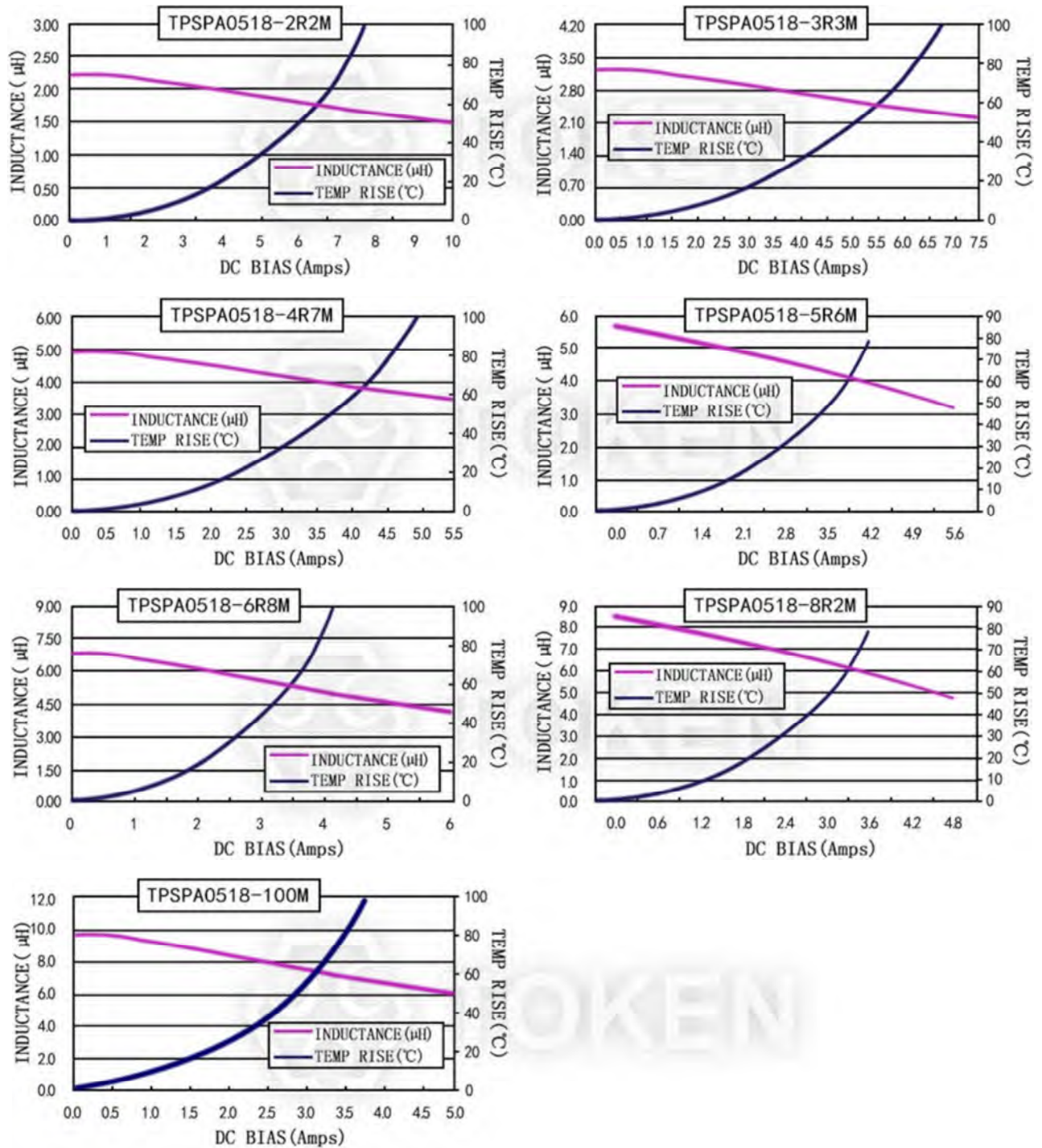
characteristics TPSPA0518-***M Series
