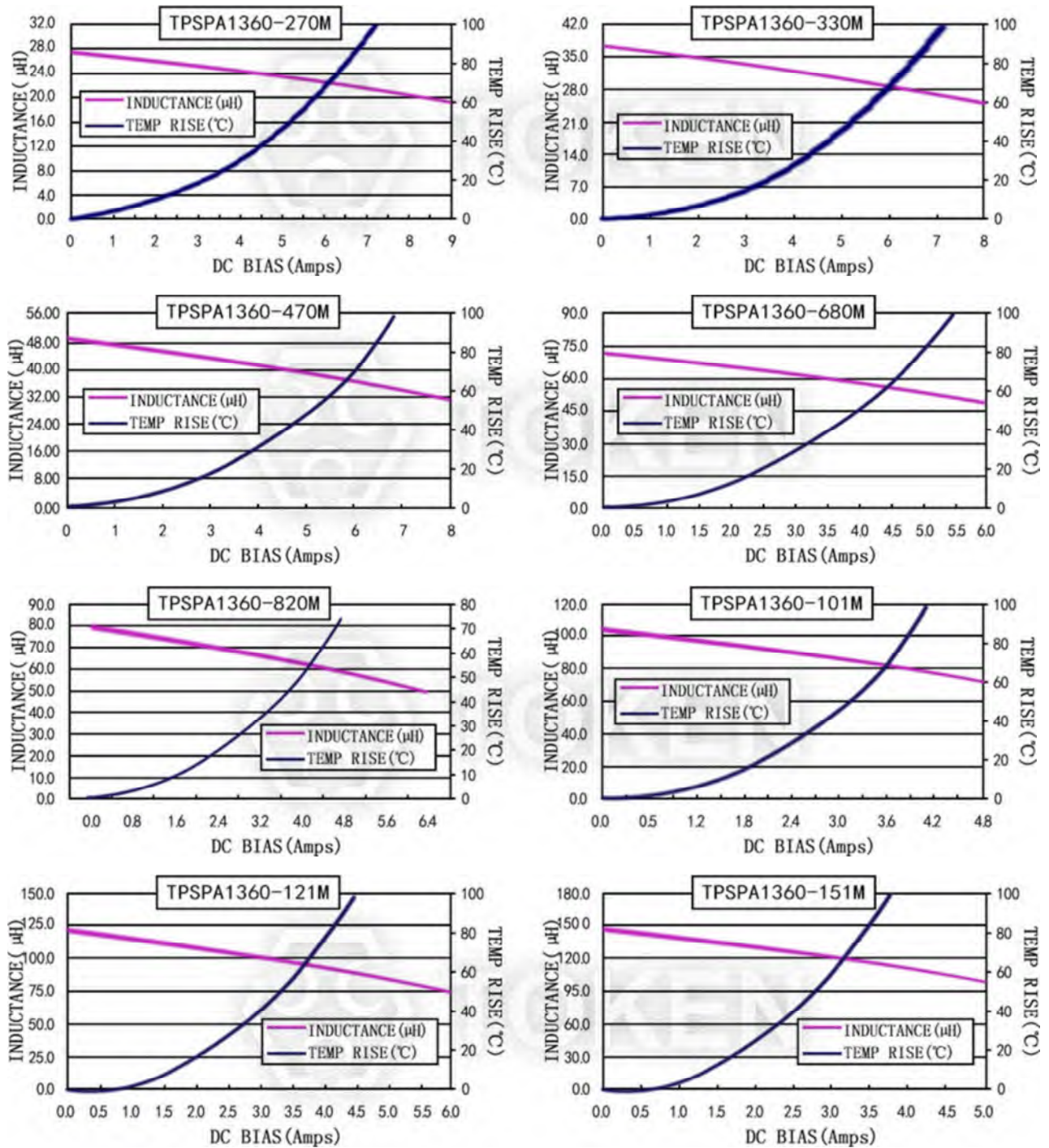
characteristics TPSPA1360-***M Series
