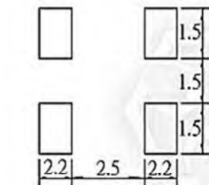
7060 PAD LAYOUT
