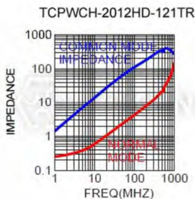
1.TDR Impedance Curve (For HDMI)
