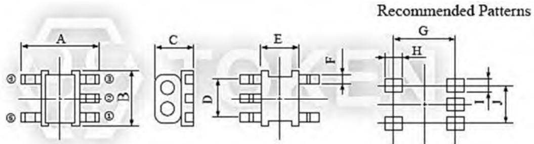
Surface mount RF Balun Transformer (TCB5F) Dimensions
