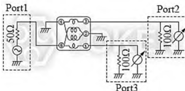
SMD Balun Transformer (TCB5FL) Test Circuit
