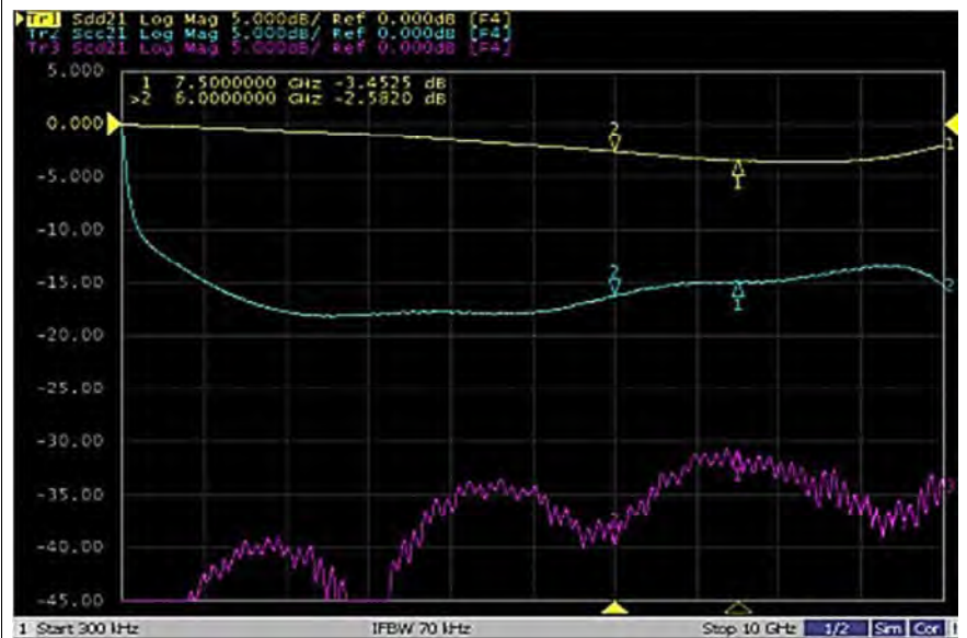
2.Insertion Loss Curve (For HDMI)
