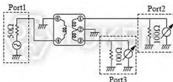
(TCB5F - 458PT) Test Circuit
