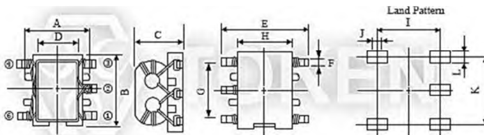
SMD Common Mode RF Balun Transformer (TCB4F) Dimensions
