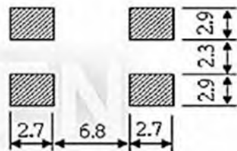
1211 PAD LAYOUT
